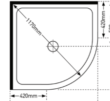
CURVED 1000 X 1000
