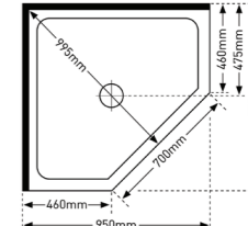
ANGLED 950 X 950
