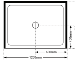
3 SIDED 1200 X 900
