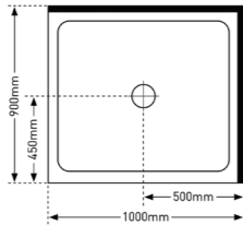
2 SIDED 1000 X 900 LEFT HAND
