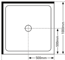
2 SIDED 1000 X 1000
