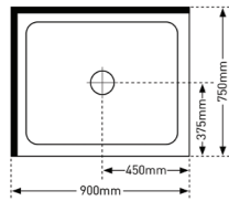
2 SIDED 900 X 750 RIGHT HAND
