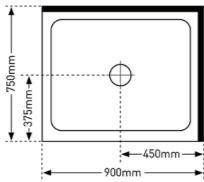
2 SIDED 900 X 750 LEFT HAND
