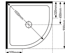
CURVED 900 X 900
