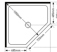
ANGLED 1000 X 1000
