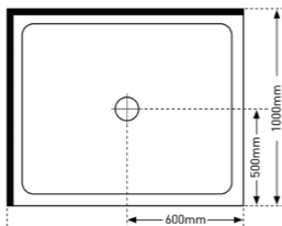
2 SIDED 1200 X 1000 RIGHT HAND
