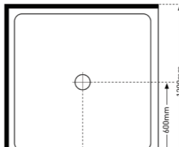
2 SIDED 1200 X 1200
