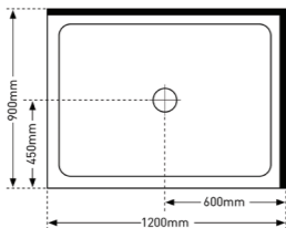
2 SIDED 1200 X 900 LEFT HAND
