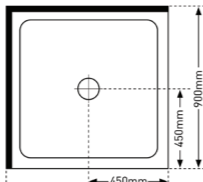
2 SIDED 900 X 900
